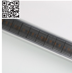
AK Clear Cover + 23° (KKLN-03) lens + Micro Louvre W25.0/H30.6mm (W0.98/H1.20")
